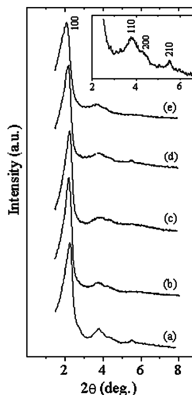
Figure 1. XRD patterns of as-synthesized: (a) HMA, (b) VHMA(200), (c) VHMA(100), (d) VHMA(50) and (e) VHMA(25).
